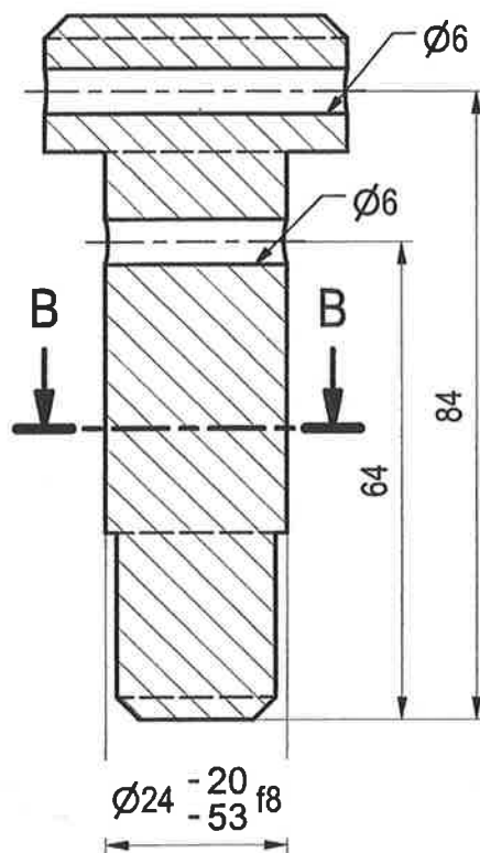
B-B (1:1)
