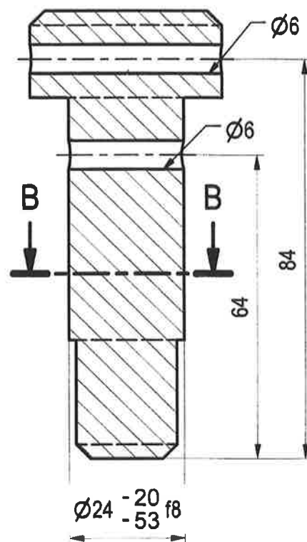
B-B (1:1)
